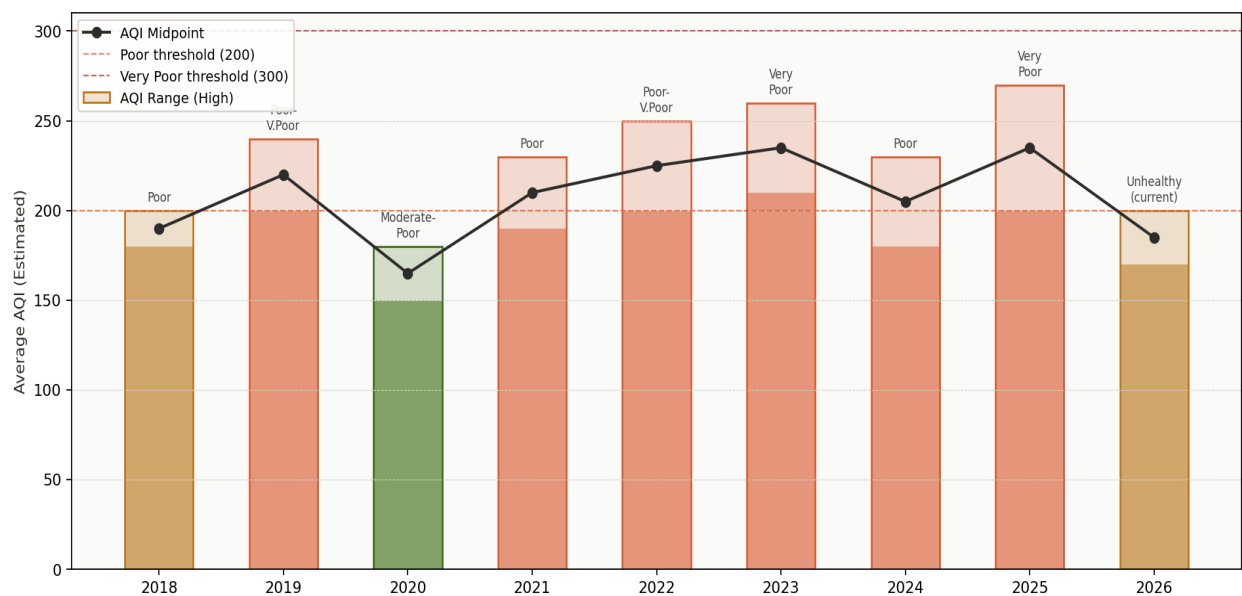
Baghpat / Western UP - AQI Trend (2018-2026)
